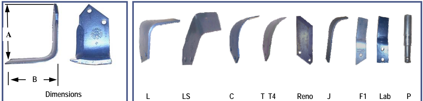
Blades for tractor mounted Rotavators (All measurements expressed in mm unless otherwise shown)
